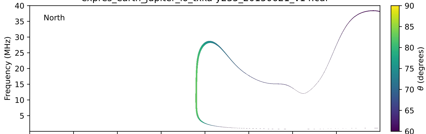
expres_earth_jupiter_io_txka-y235_20150621_v14.cdf
