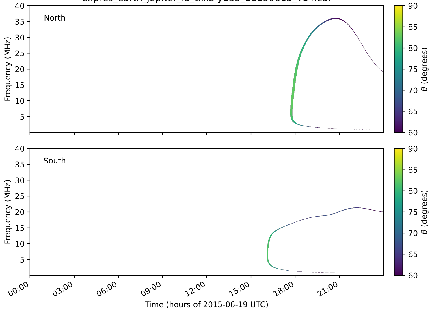
expres_earth_jupiter_io_txka-y235_20150619_v14.cdf
