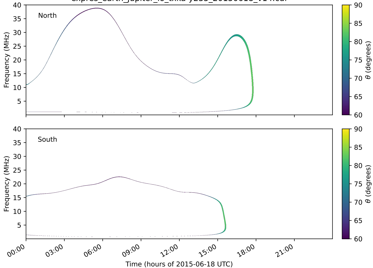
expres_earth_jupiter_io_txka-y235_20150618_v14.cdf
