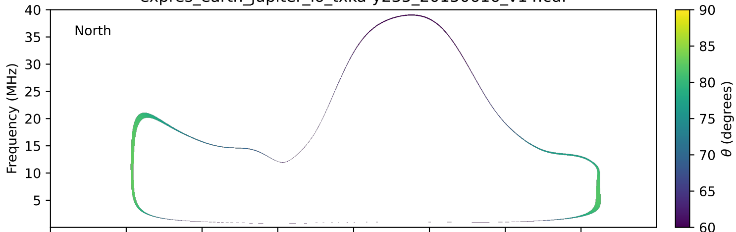
expres_earth_jupiter_io_txka-y235_20150616_v14.cdf
