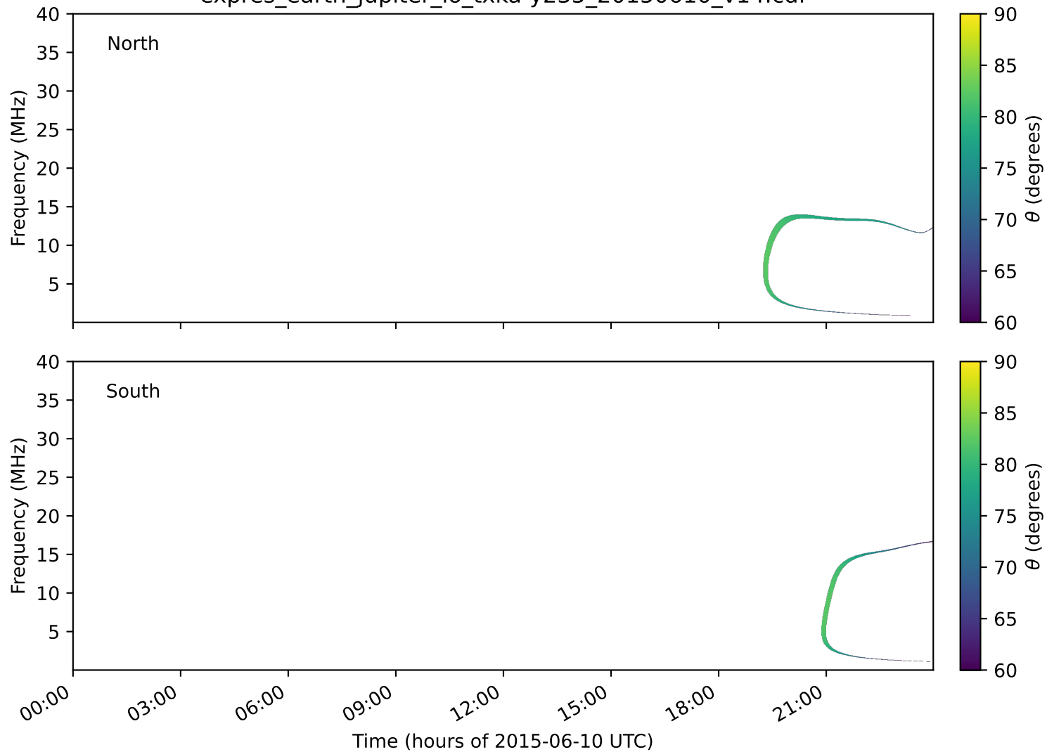
expres_earth_jupiter_io_txka-y235_20150610_v14.cdf
