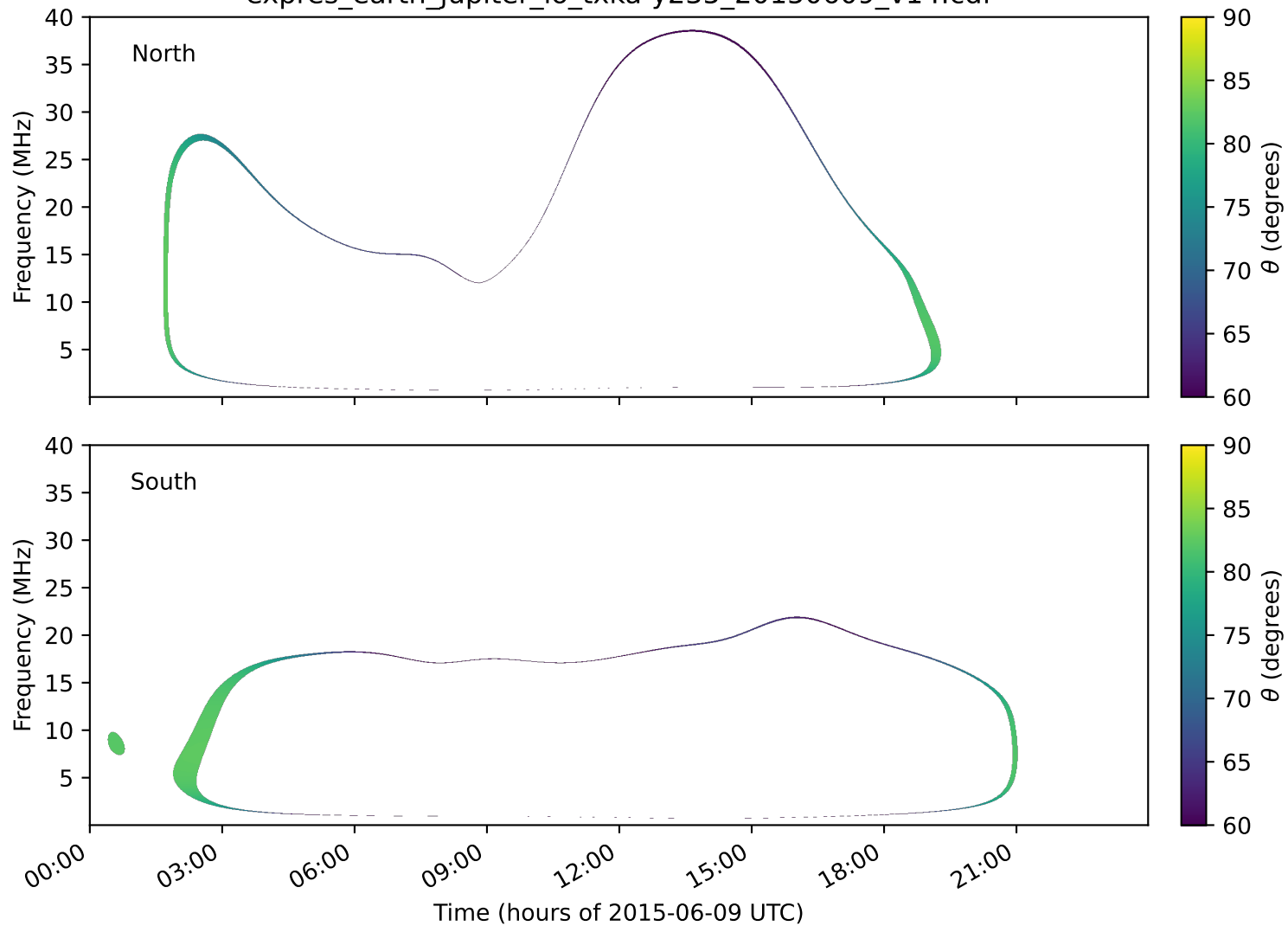
expres_earth_jupiter_io_txka-y235_20150609_v14.cdf
