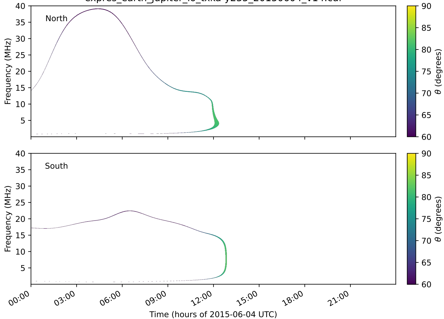
expres_earth_jupiter_io_txka-y235_20150604_v14.cdf
