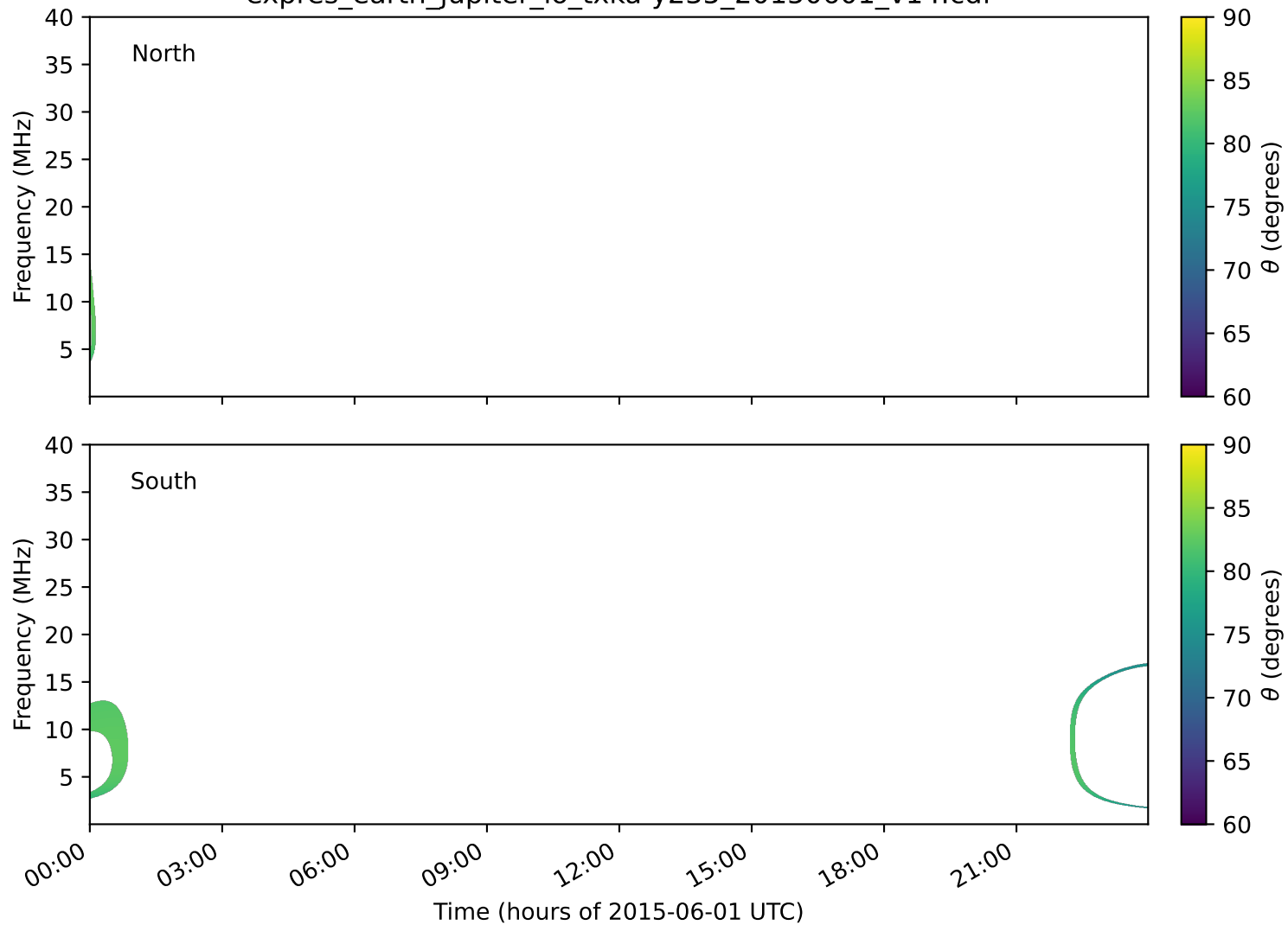
expres_earth_jupiter_io_txka-y235_20150601_v14.cdf
