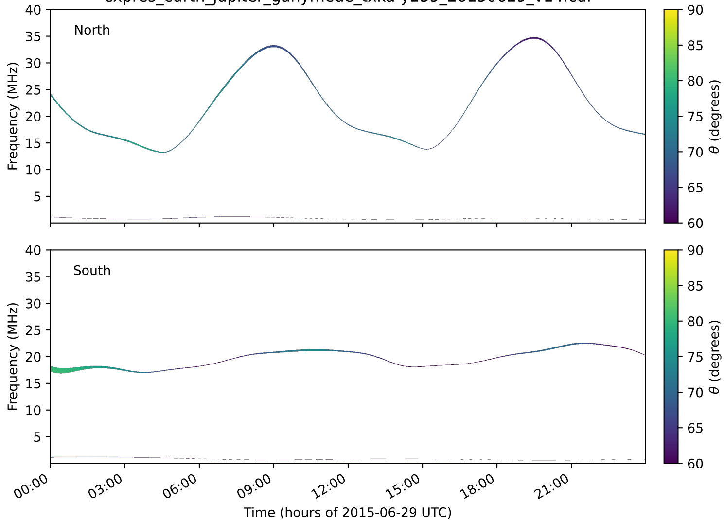
expres_earth_jupiter_ganymede_txka-y235_20150629_v14.cdf
