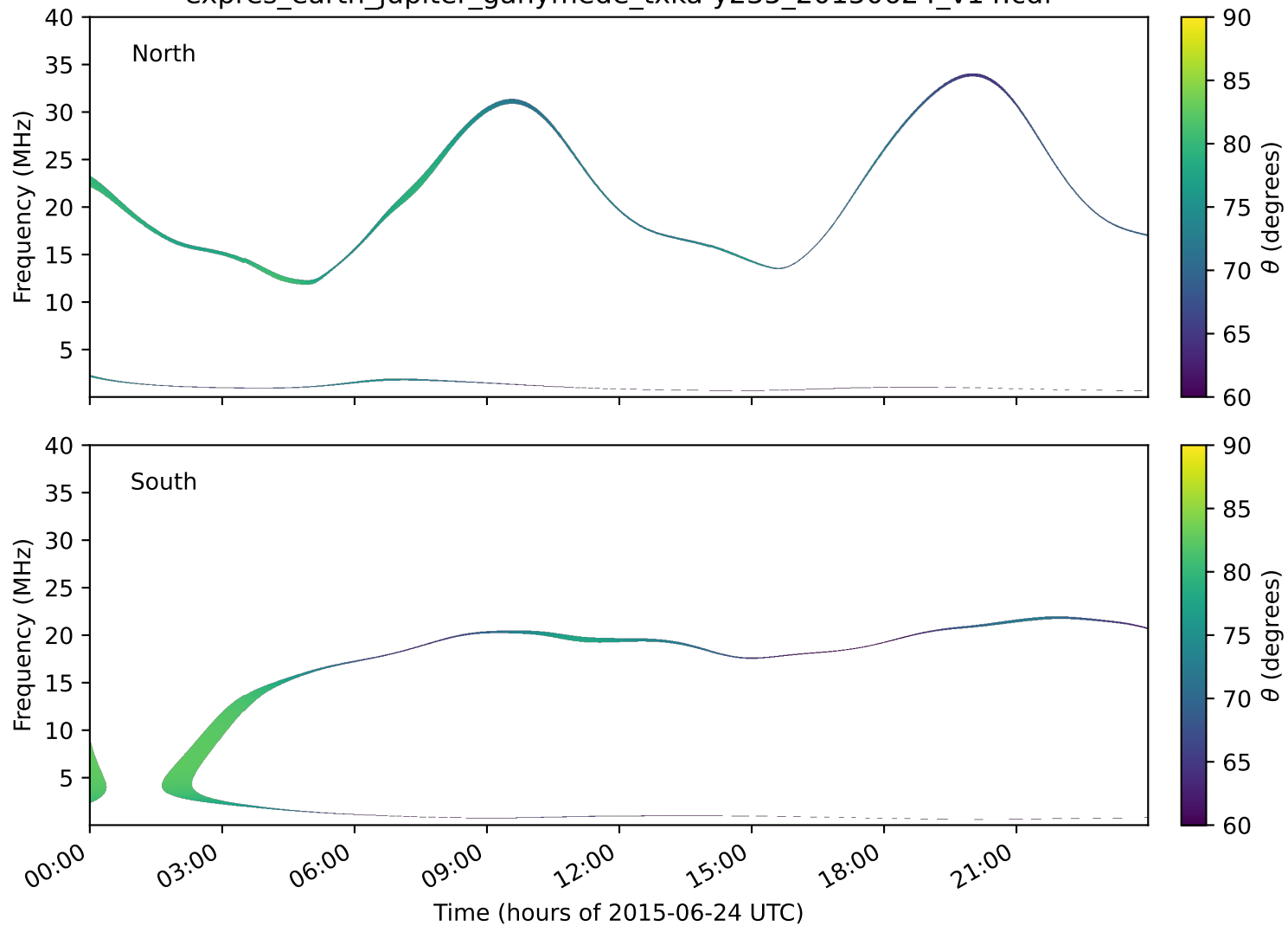
expres_earth_jupiter_ganymede_txka-y235_20150624_v14.cdf
