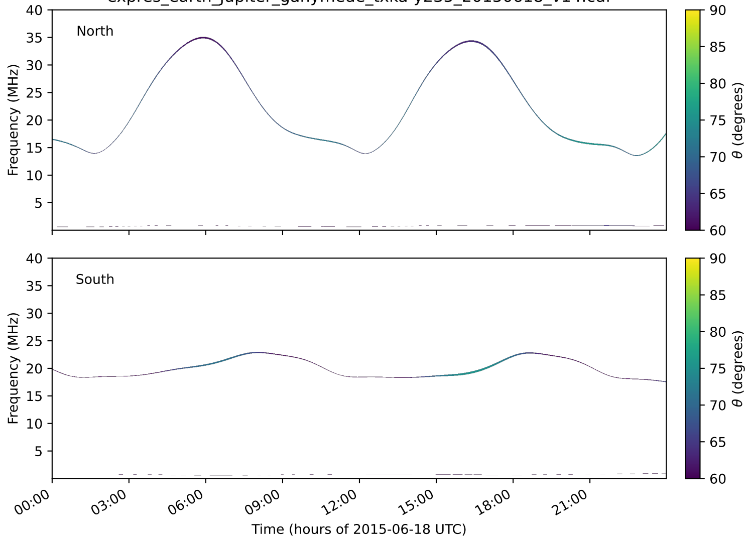
expres_earth_jupiter_ganymede_txka-y235_20150618_v14.cdf
