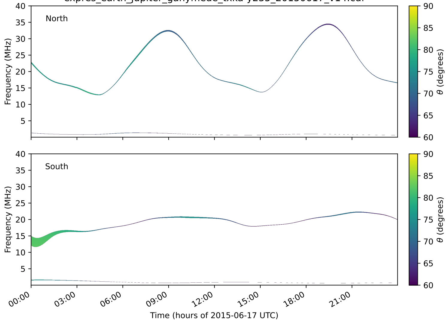
expres_earth_jupiter_ganymede_txka-y235_20150617_v14.cdf
