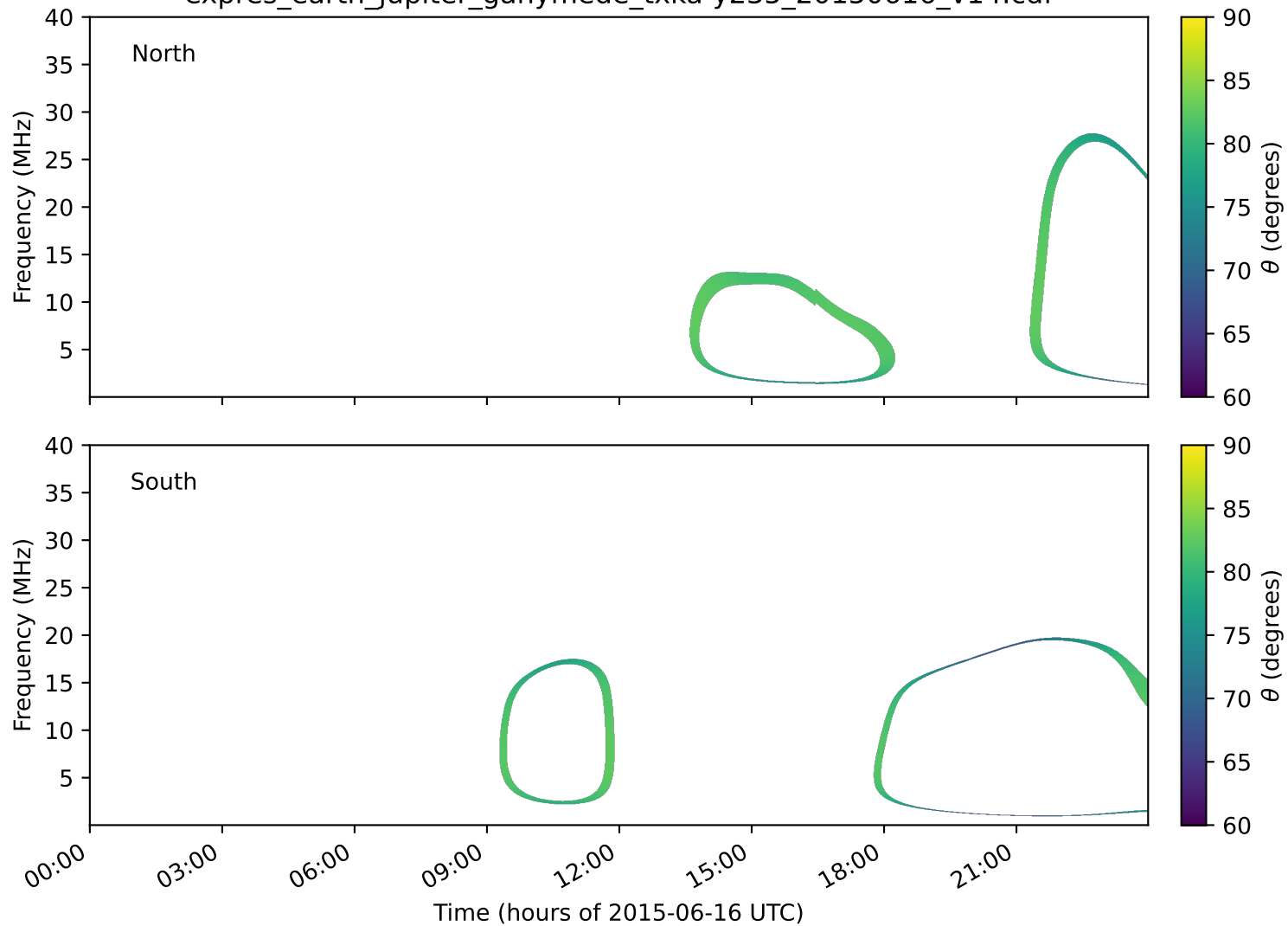
expres_earth_jupiter_ganymede_txka-y235_20150616_v14.cdf
