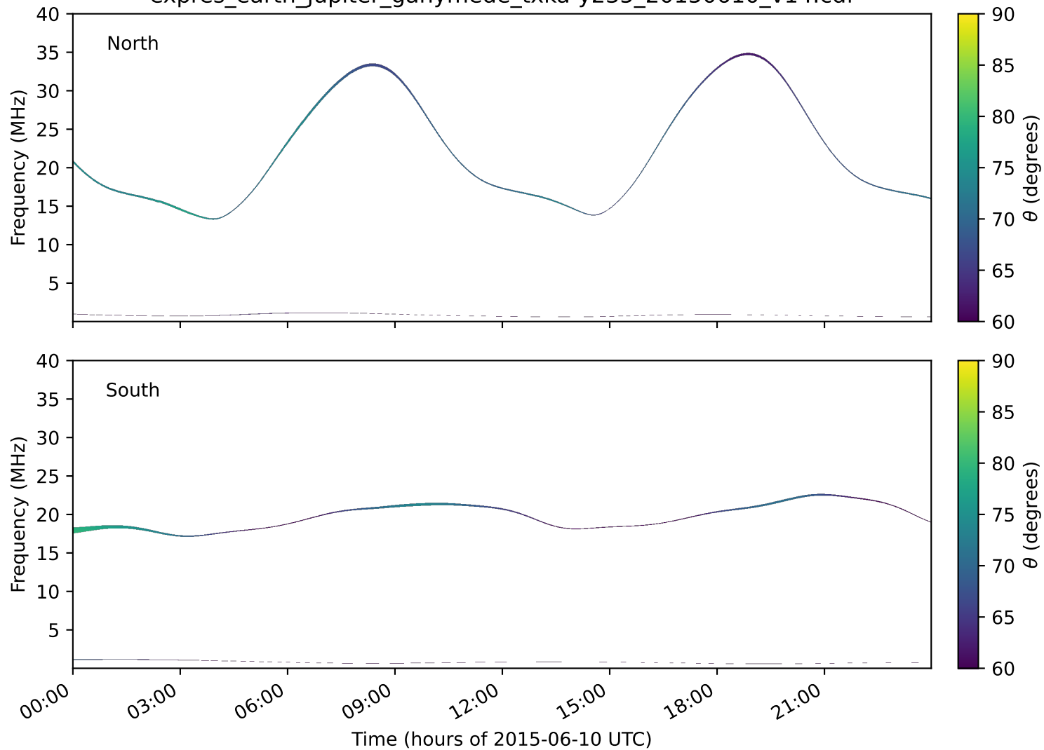
expres_earth_jupiter_ganymede_txka-y235_20150610_v14.cdf
