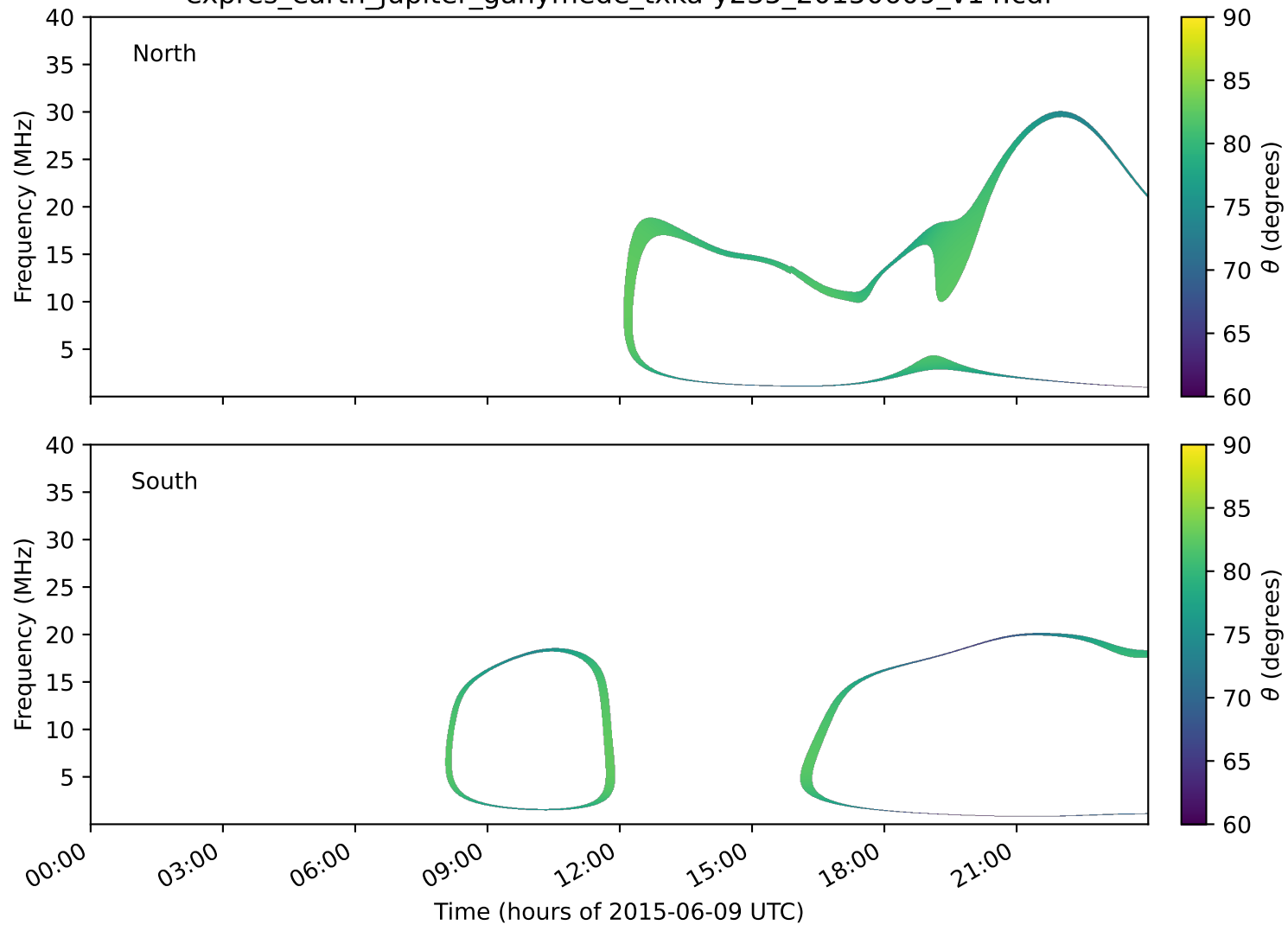
expres_earth_jupiter_ganymede_txka-y235_20150609_v14.cdf
