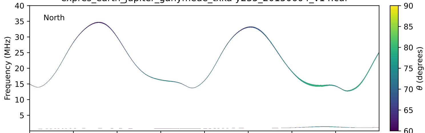
expres_earth_jupiter_ganymede_txka-y235_20150604_v14.cdf
