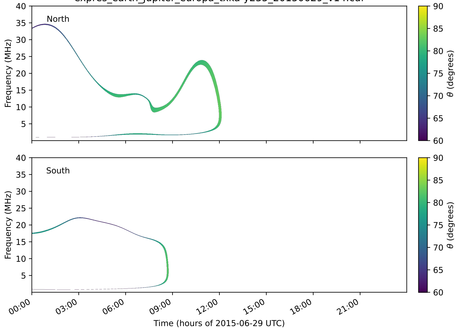
expres_earth_jupiter_europa_txka-y235_20150629_v14.cdf
