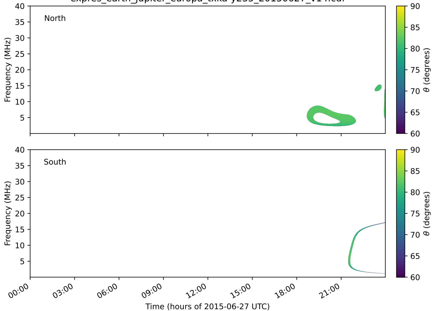
expres_earth_jupiter_europa_txka-y235_20150627_v14.cdf
