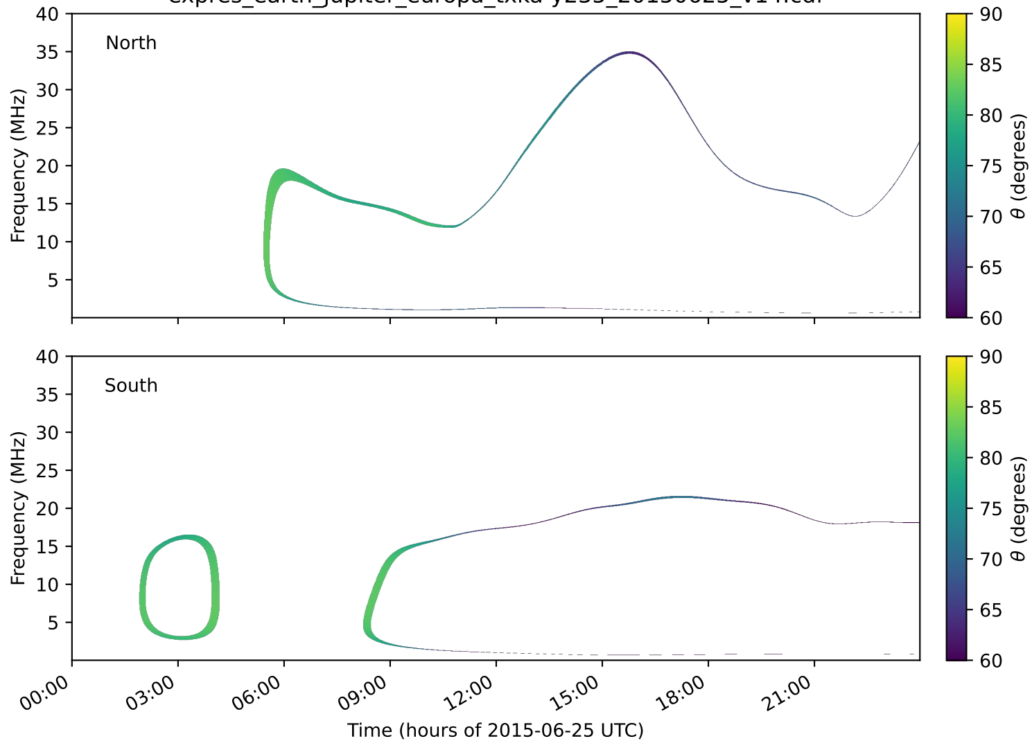
expres_earth_jupiter_europa_txka-y235_20150625_v14.cdf
