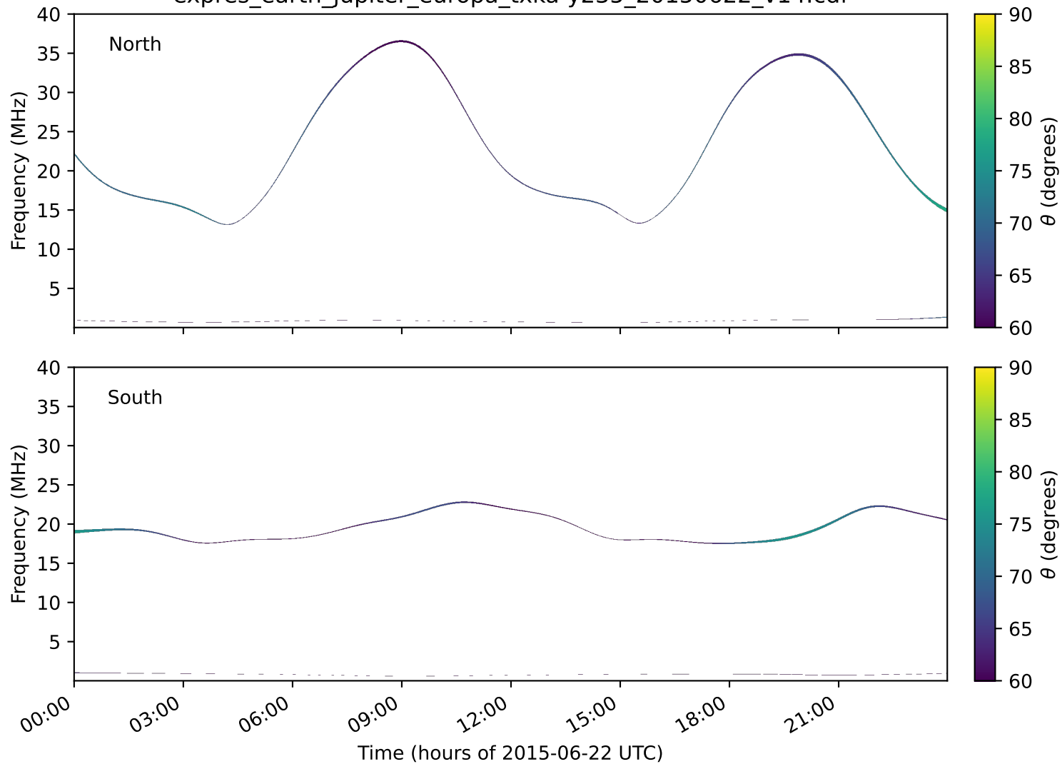
expres_earth_jupiter_europa_txka-y235_20150622_v14.cdf
