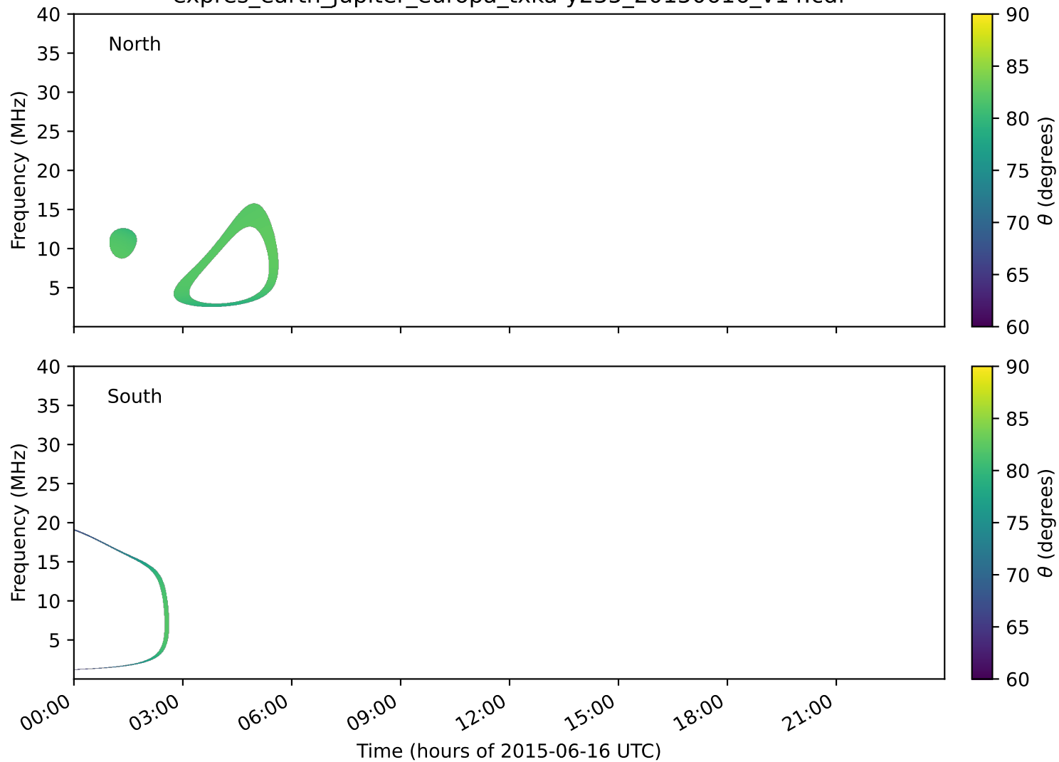
expres_earth_jupiter_europa_txka-y235_20150616_v14.cdf
