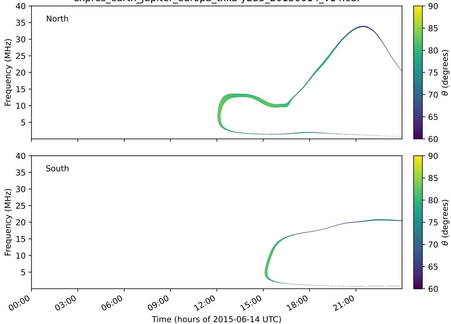
expres_earth_jupiter_europa_txka-y235_20150614_v14.cdf
