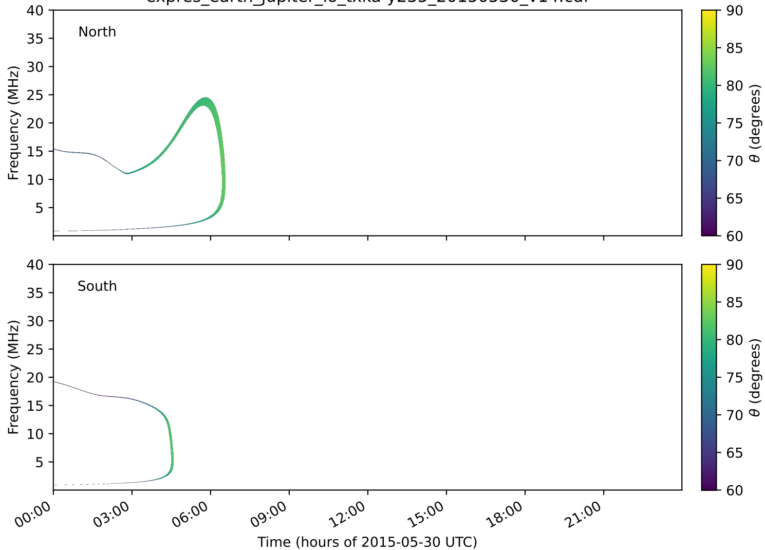
expres_earth_jupiter_io_txka-y235_20150530_v14.cdf
