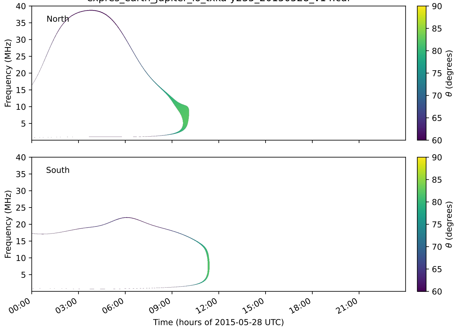
expres_earth_jupiter_io_txka-y235_20150528_v14.cdf
