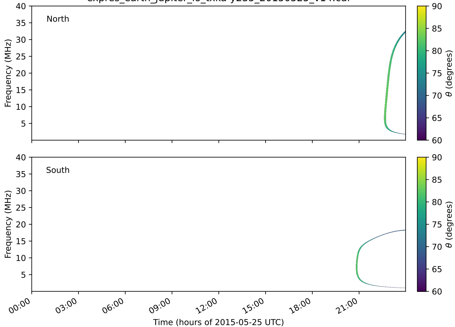
expres_earth_jupiter_io_txka-y235_20150525_v14.cdf
