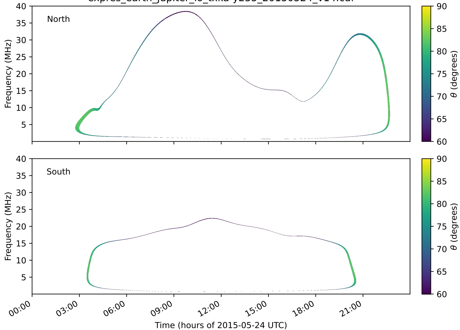
expres_earth_jupiter_io_txka-y235_20150524_v14.cdf
