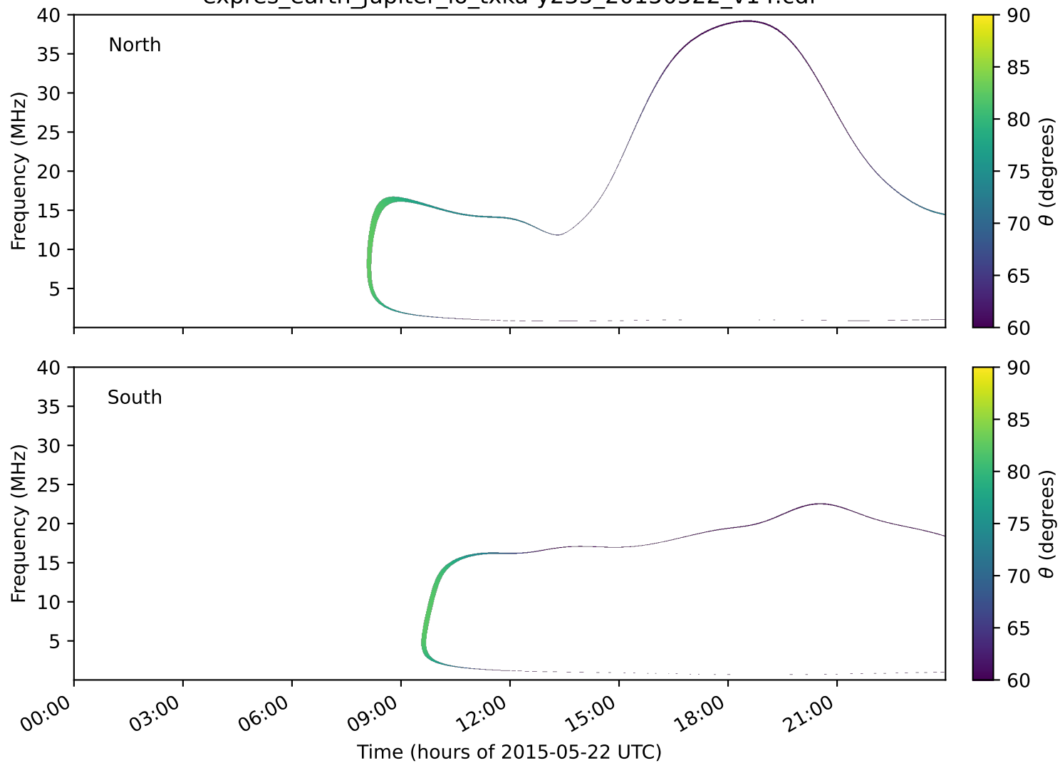
expres_earth_jupiter_io_txka-y235_20150522_v14.cdf
