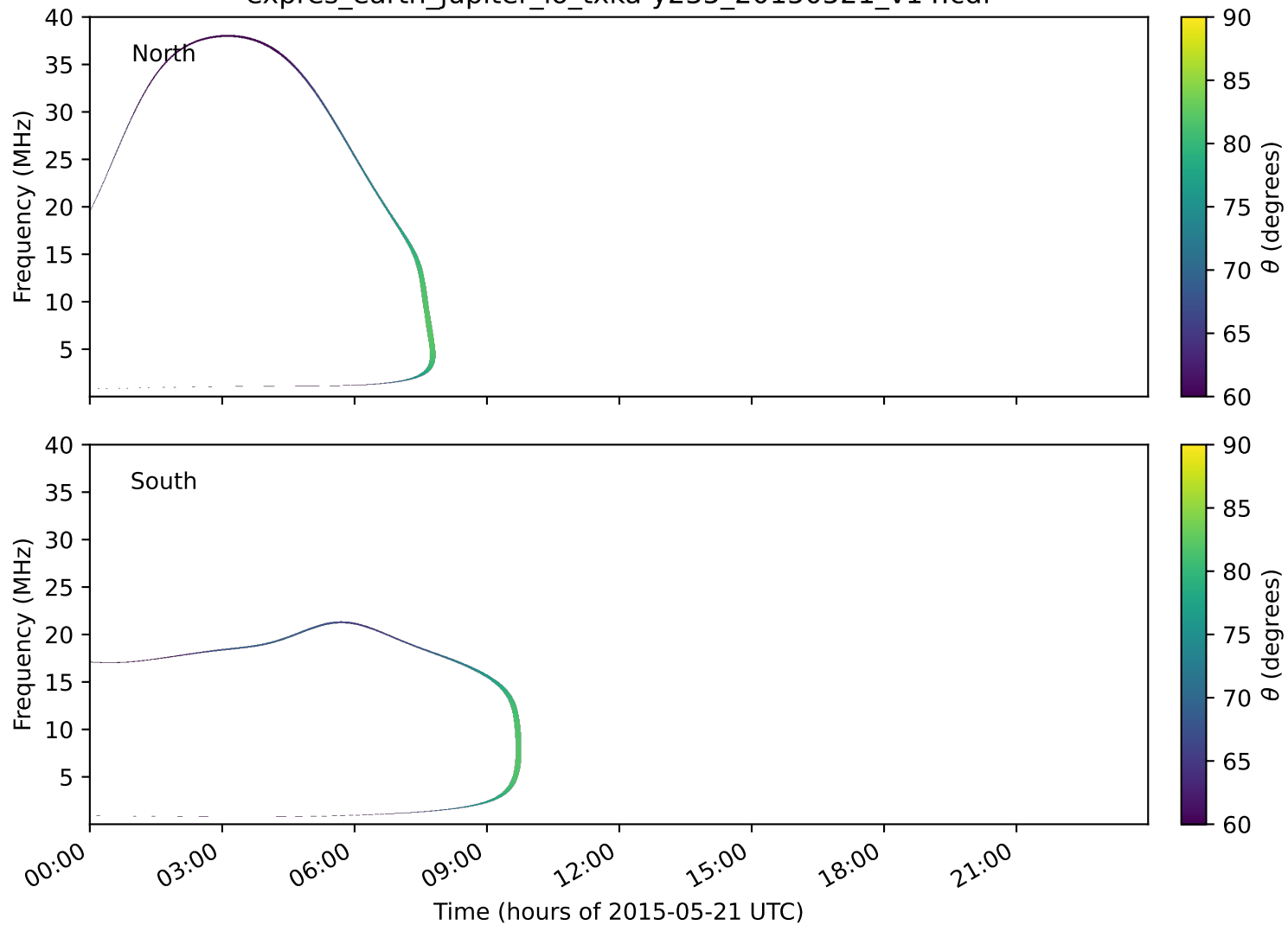
expres_earth_jupiter_io_txka-y235_20150521_v14.cdf
