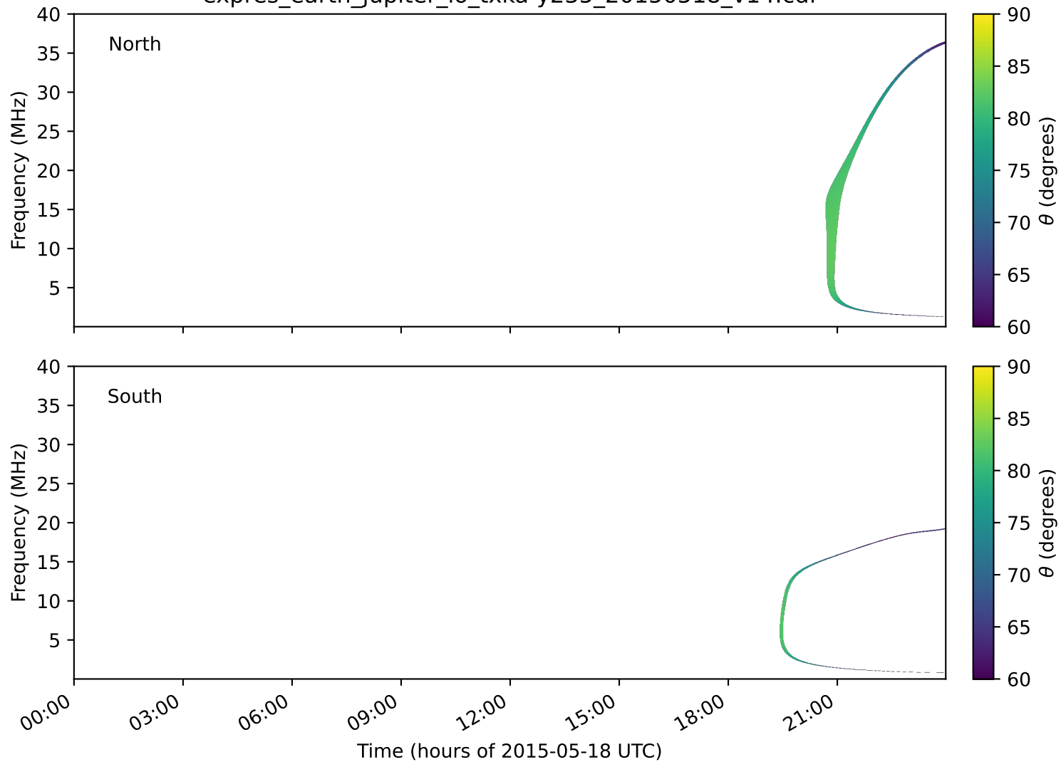
expres_earth_jupiter_io_txka-y235_20150518_v14.cdf
