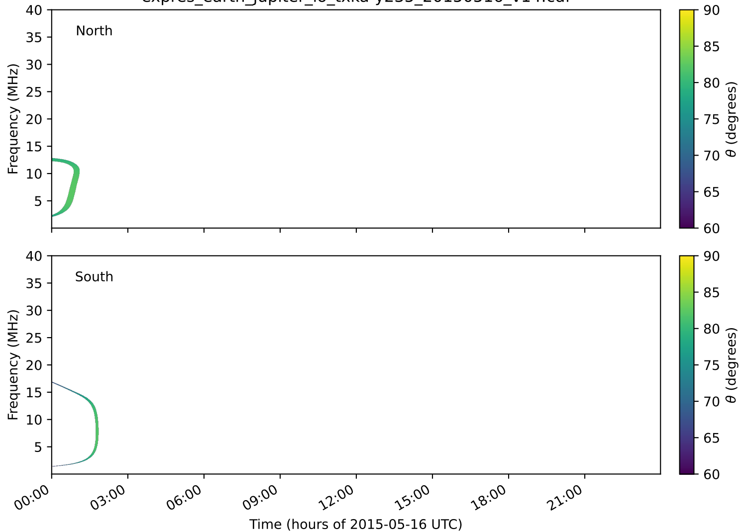
expres_earth_jupiter_io_txka-y235_20150516_v14.cdf
