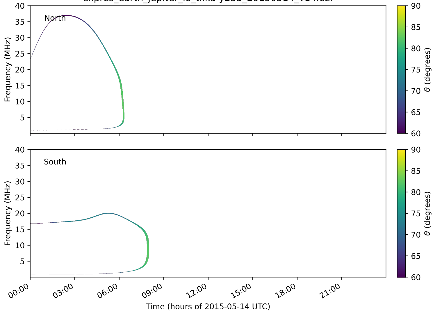
expres_earth_jupiter_io_txka-y235_20150514_v14.cdf
