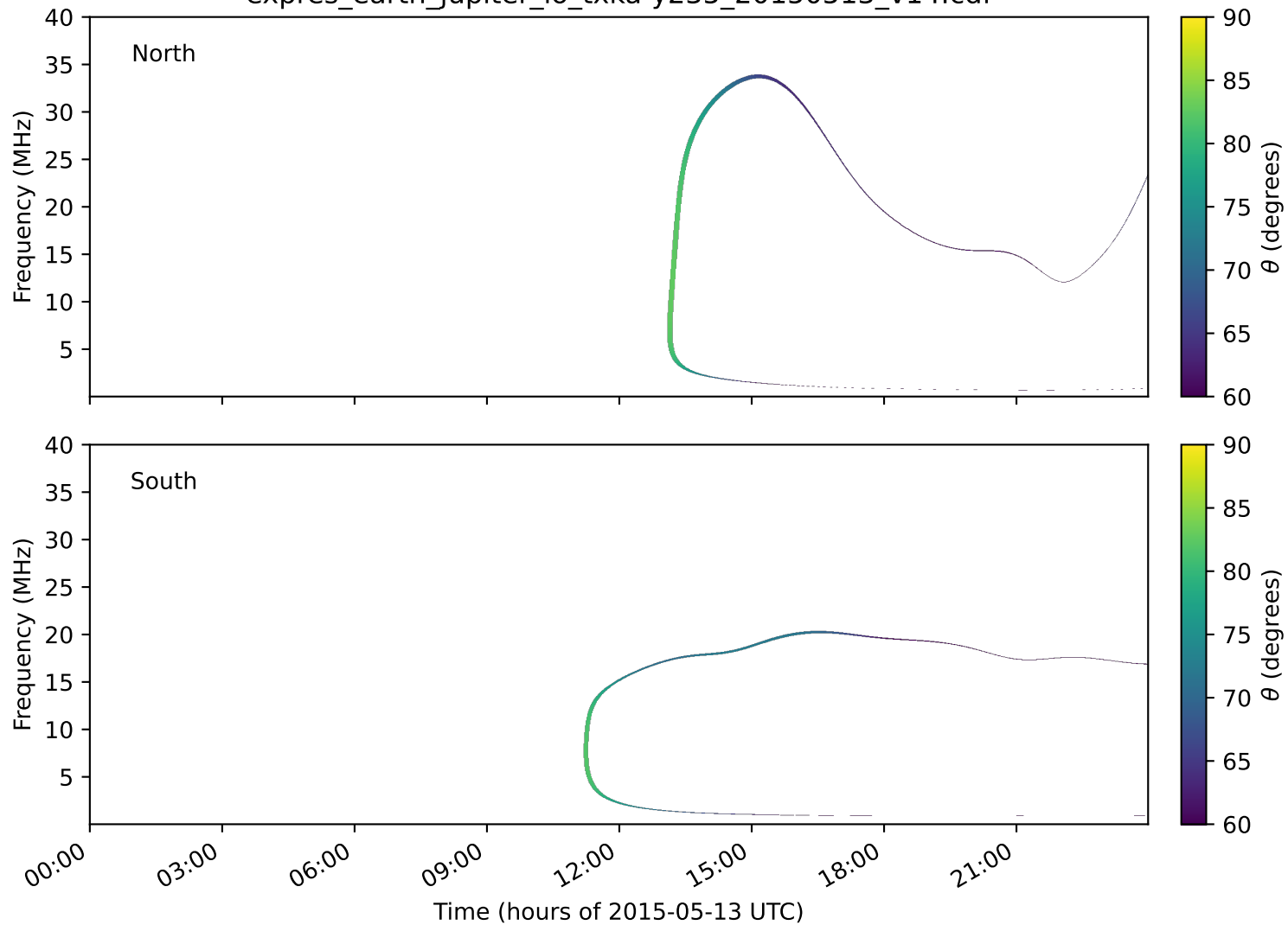
expres_earth_jupiter_io_txka-y235_20150513_v14.cdf
