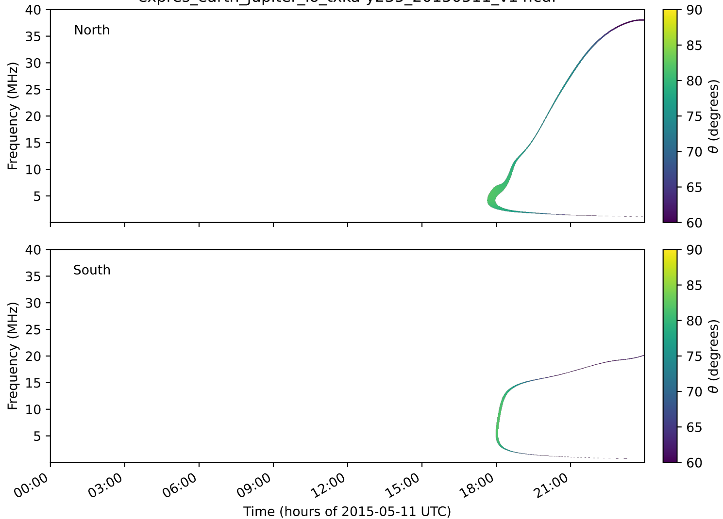
expres_earth_jupiter_io_txka-y235_20150511_v14.cdf
