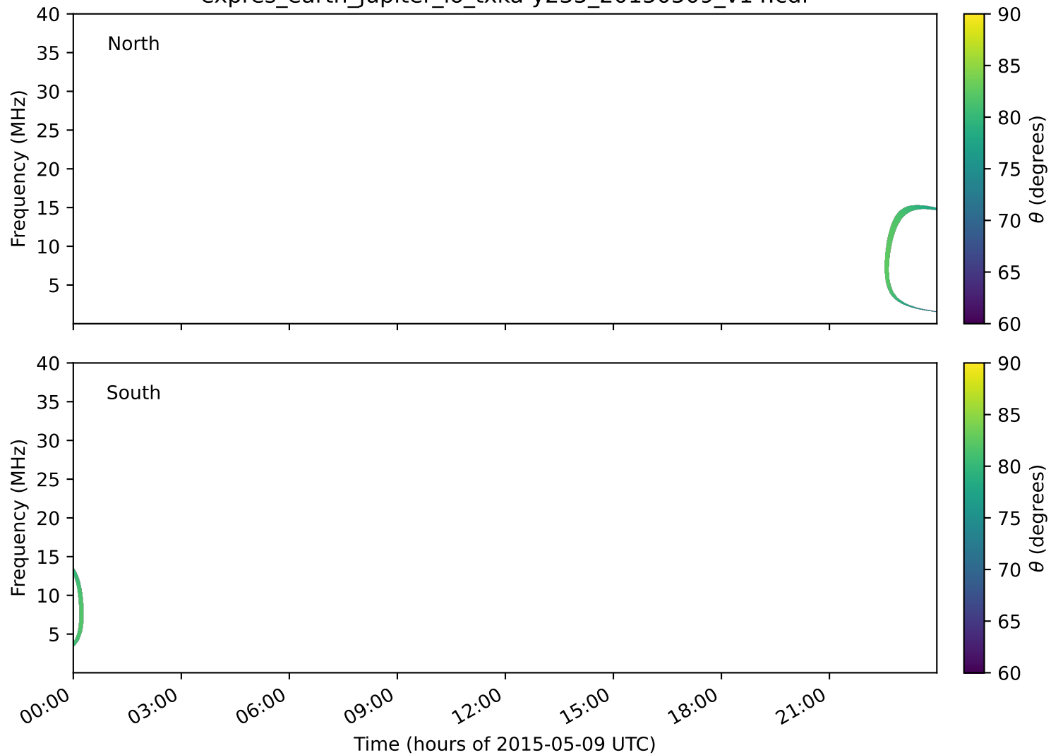
expres_earth_jupiter_io_txka-y235_20150509_v14.cdf
