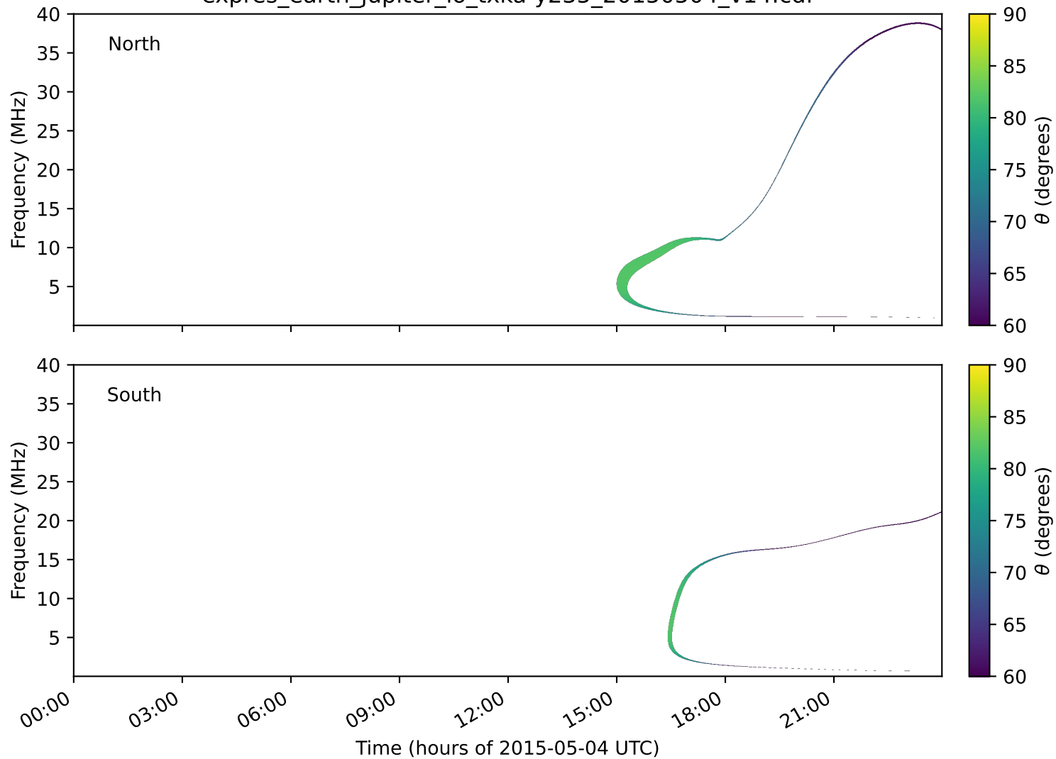
expres_earth_jupiter_io_txka-y235_20150504_v14.cdf
