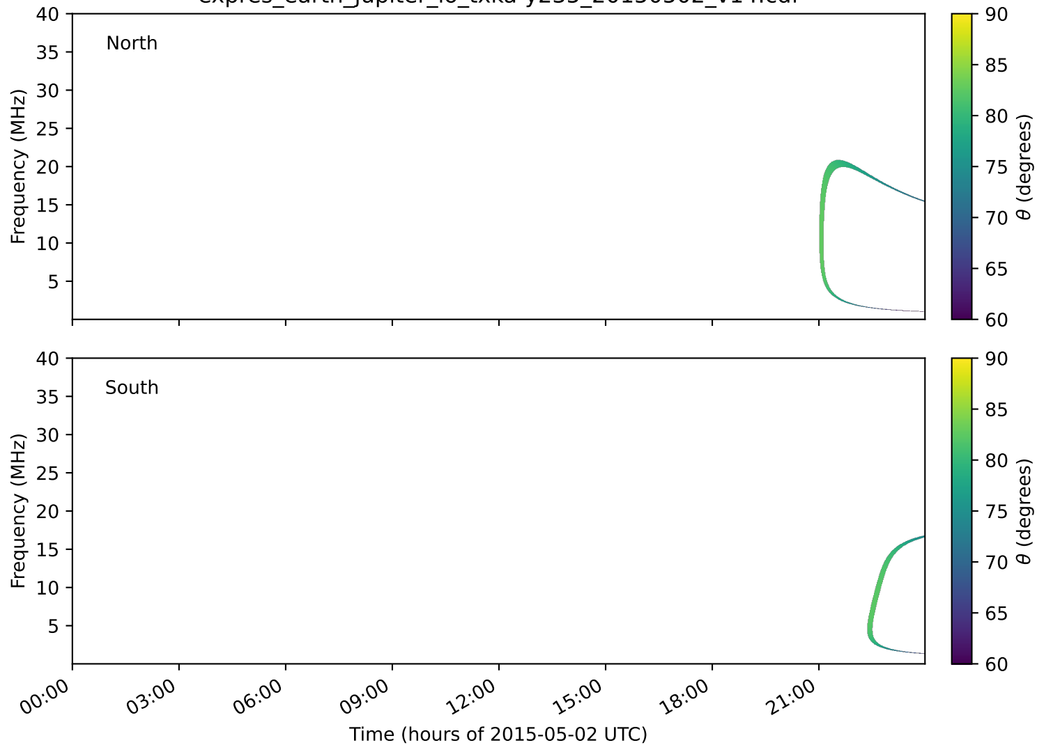
expres_earth_jupiter_io_txka-y235_20150502_v14.cdf
