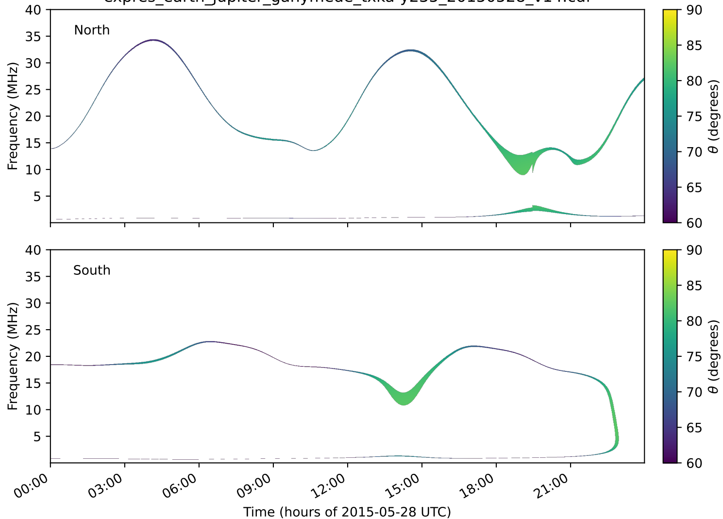
expres_earth_jupiter_ganymede_txka-y235_20150528_v14.cdf
