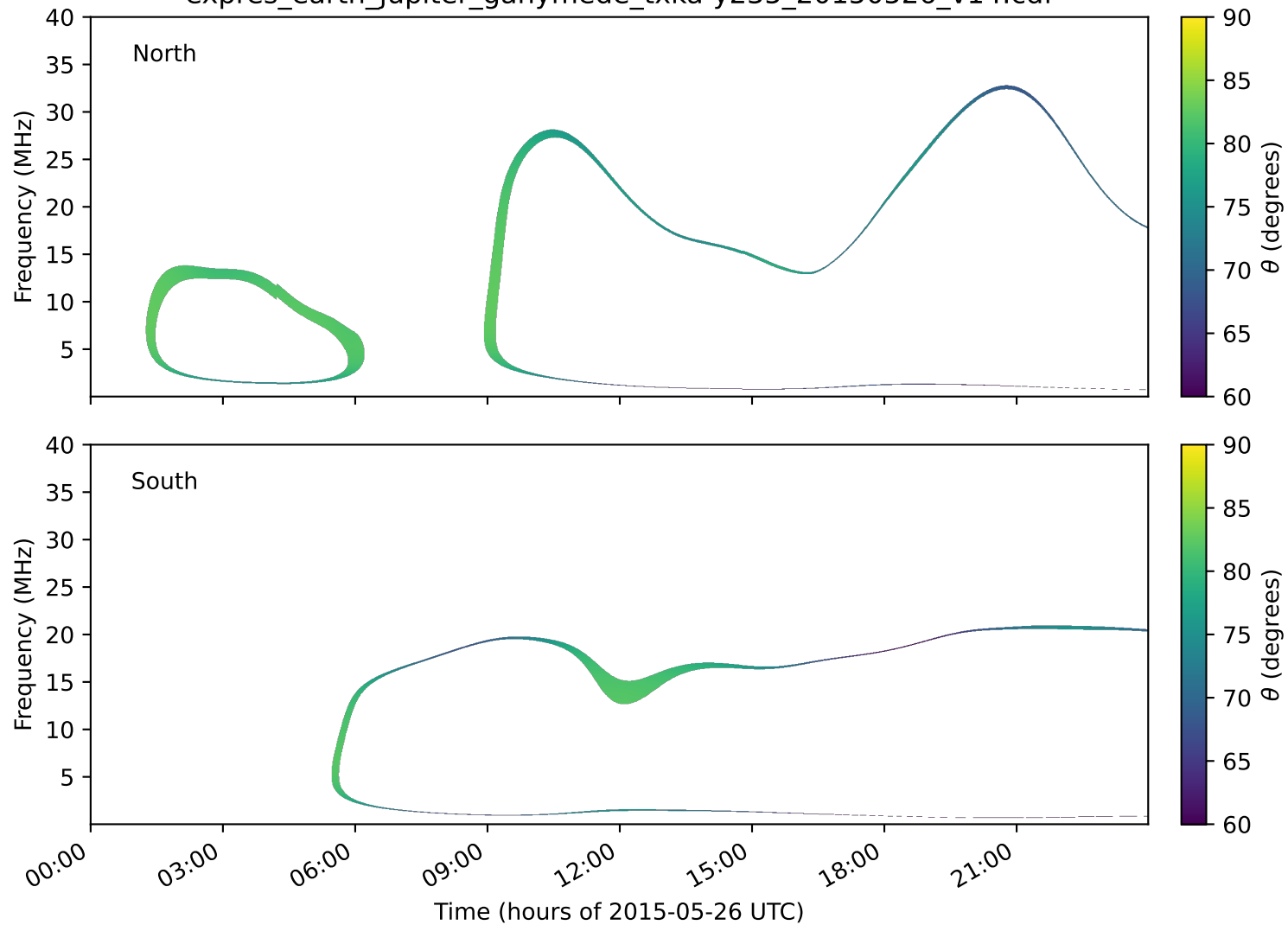
expres_earth_jupiter_ganymede_txka-y235_20150526_v14.cdf
