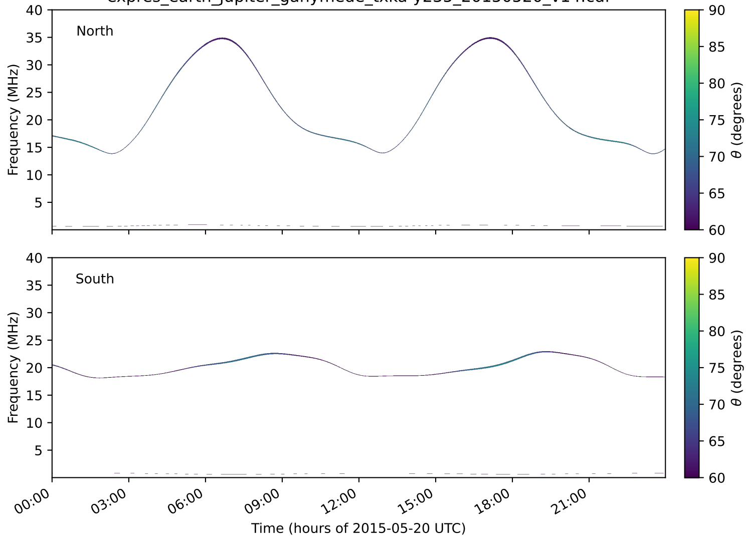
expres_earth_jupiter_ganymede_txka-y235_20150520_v14.cdf
