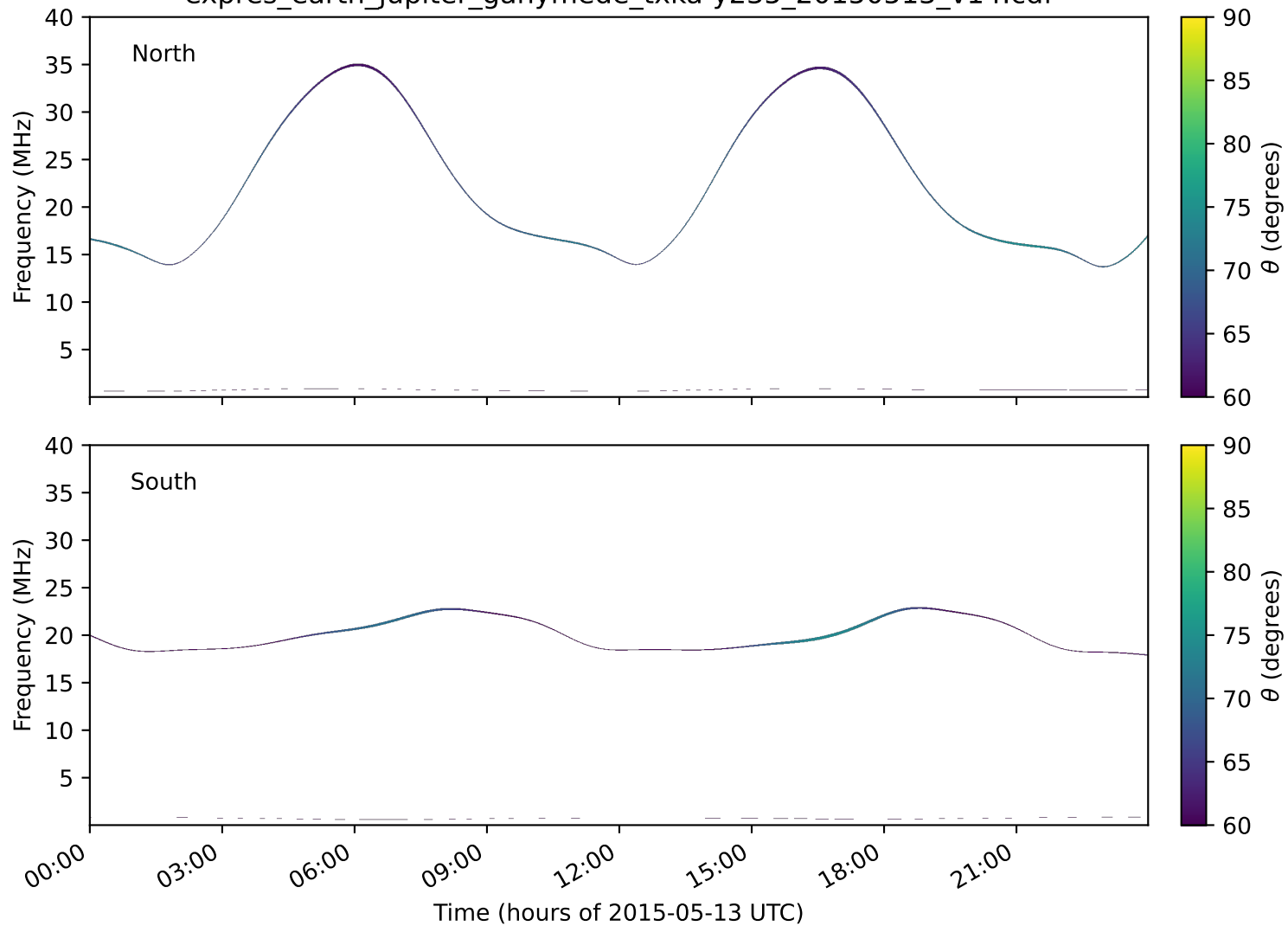
expres_earth_jupiter_ganymede_txka-y235_20150513_v14.cdf
