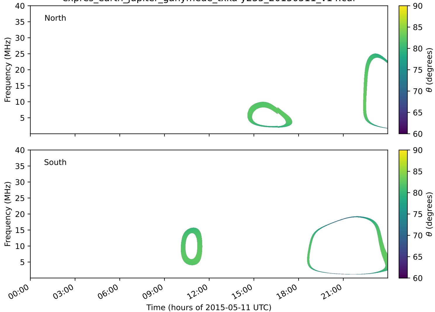
expres_earth_jupiter_ganymede_txka-y235_20150511_v14.cdf
