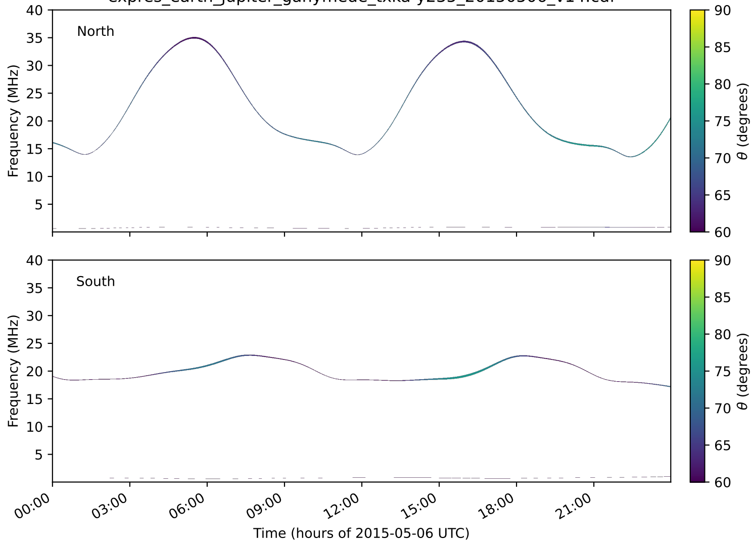
expres_earth_jupiter_ganymede_txka-y235_20150506_v14.cdf
