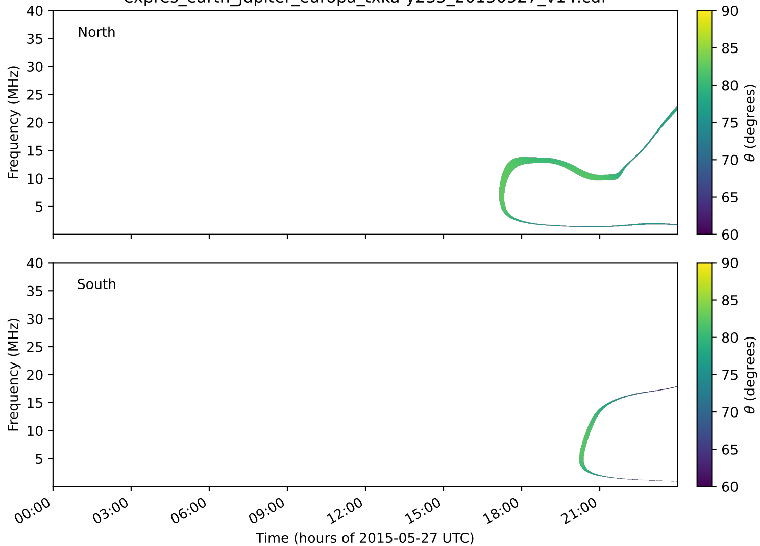
expres_earth_jupiter_europa_txka-y235_20150527_v14.cdf
