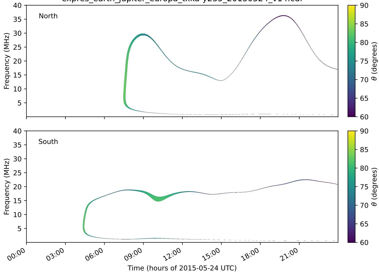
expres_earth_jupiter_europa_txka-y235_20150524_v14.cdf
