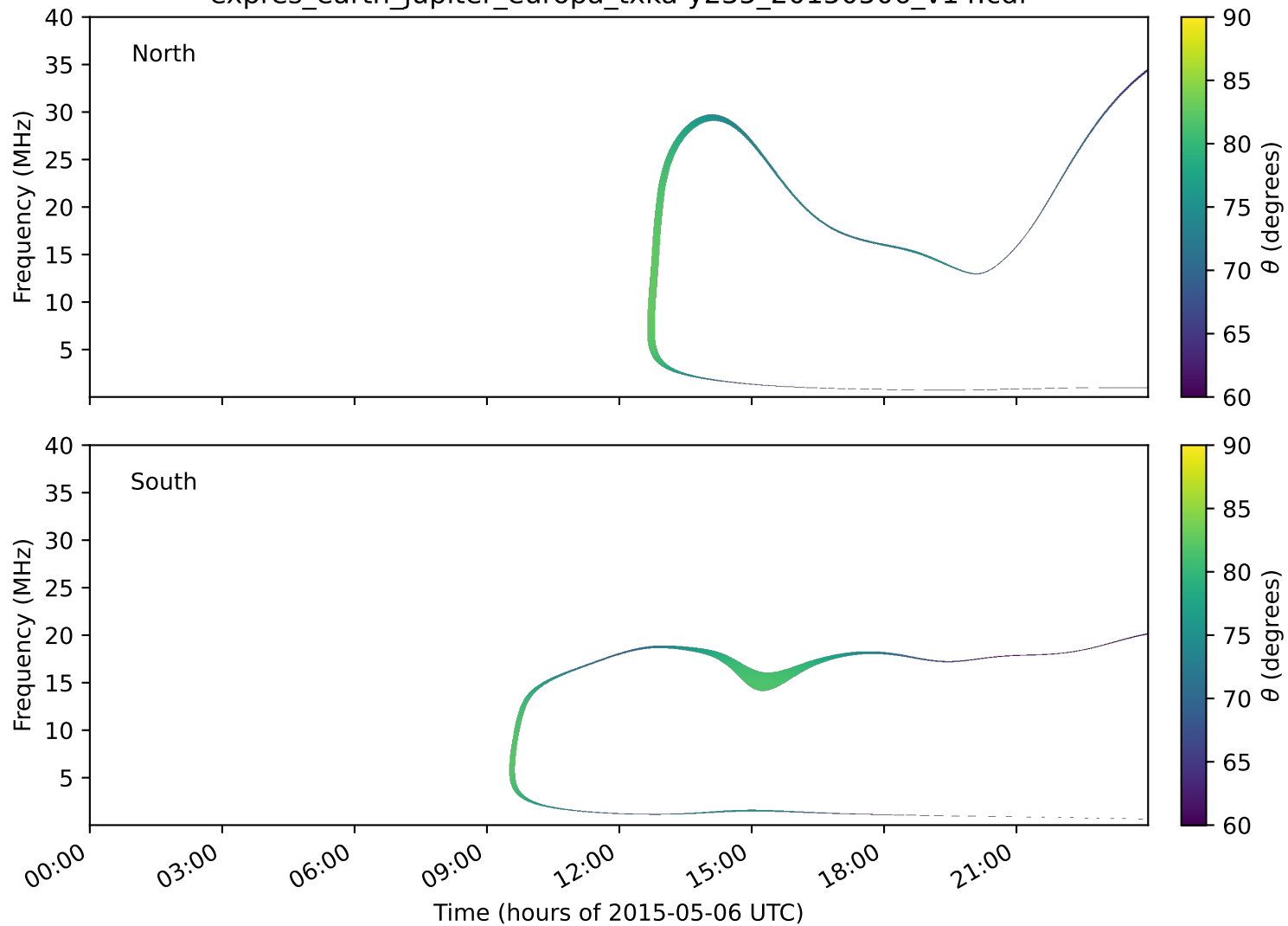
expres_earth_jupiter_europa_txka-y235_20150506_v14.cdf
