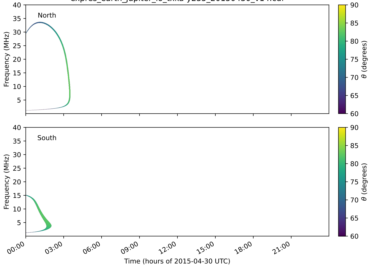
expres_earth_jupiter_io_txka-y235_20150430_v14.cdf
