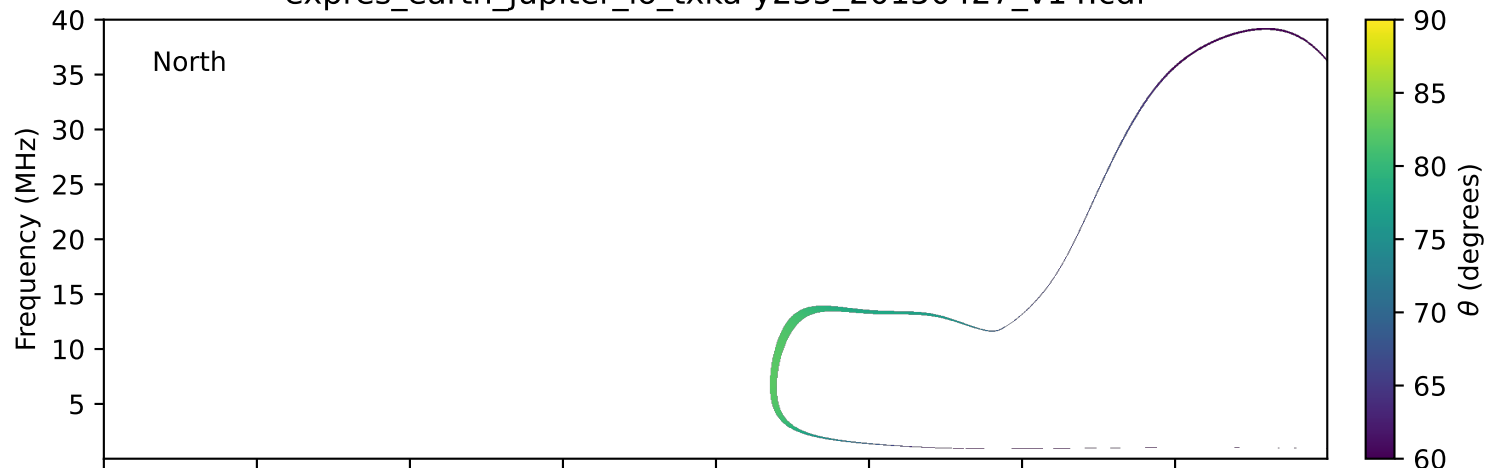
expres_earth_jupiter_io_txka-y235_20150427_v14.cdf
