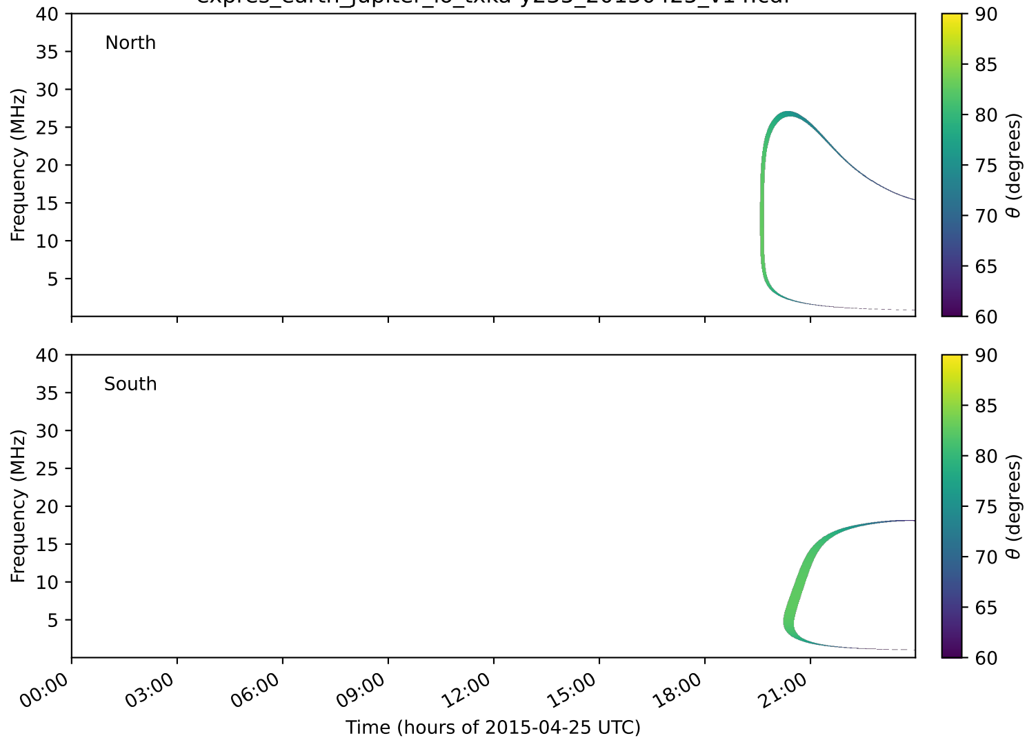
expres_earth_jupiter_io_txka-y235_20150425_v14.cdf
