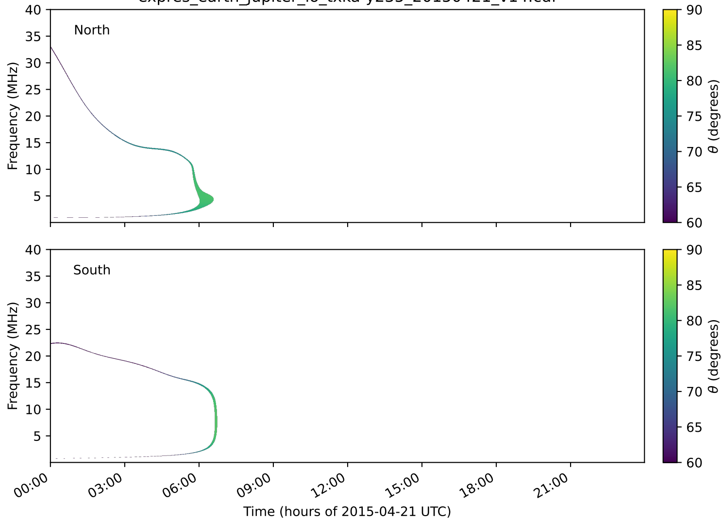
expres_earth_jupiter_io_txka-y235_20150421_v14.cdf
