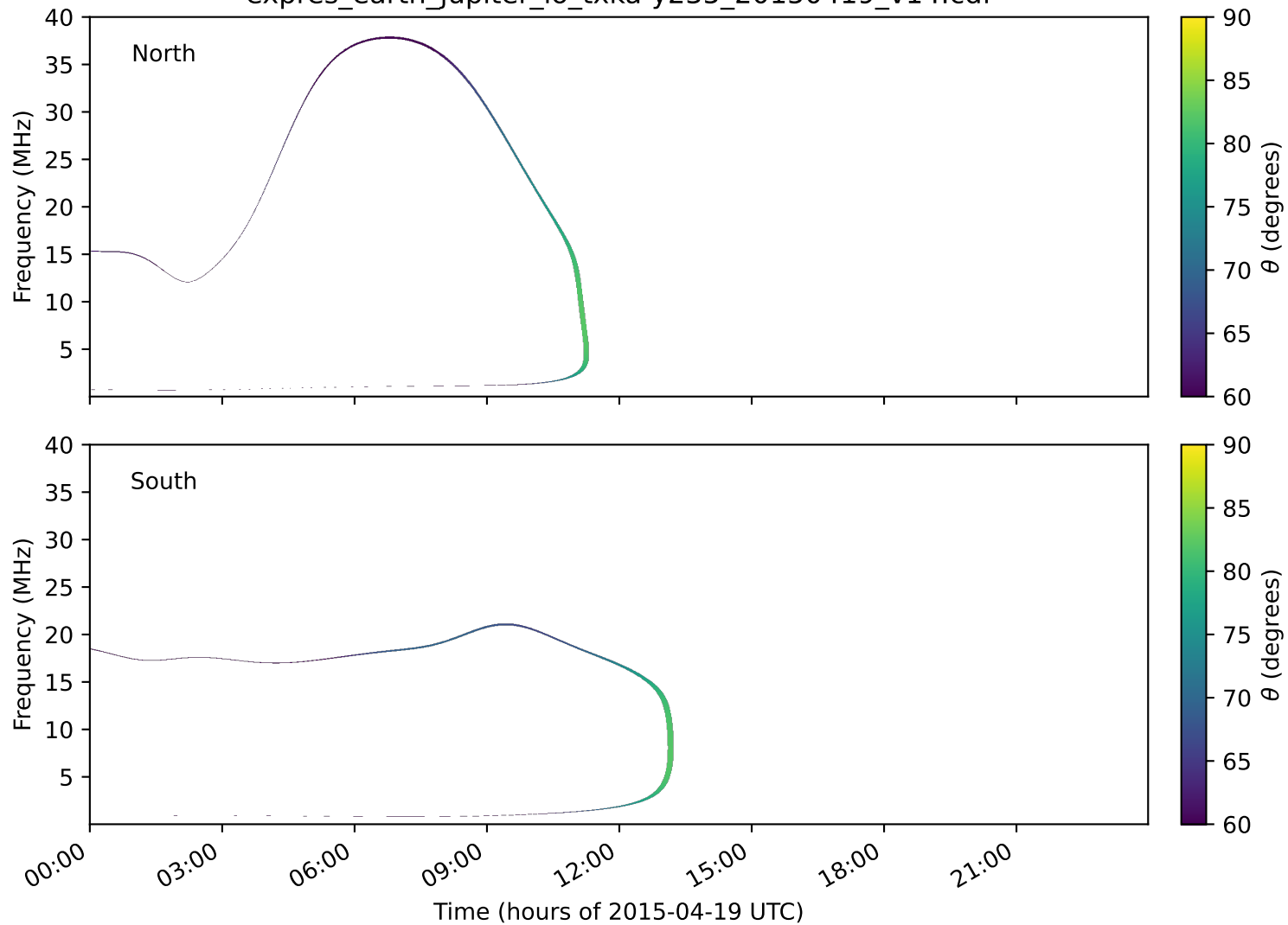
expres_earth_jupiter_io_txka-y235_20150419_v14.cdf
